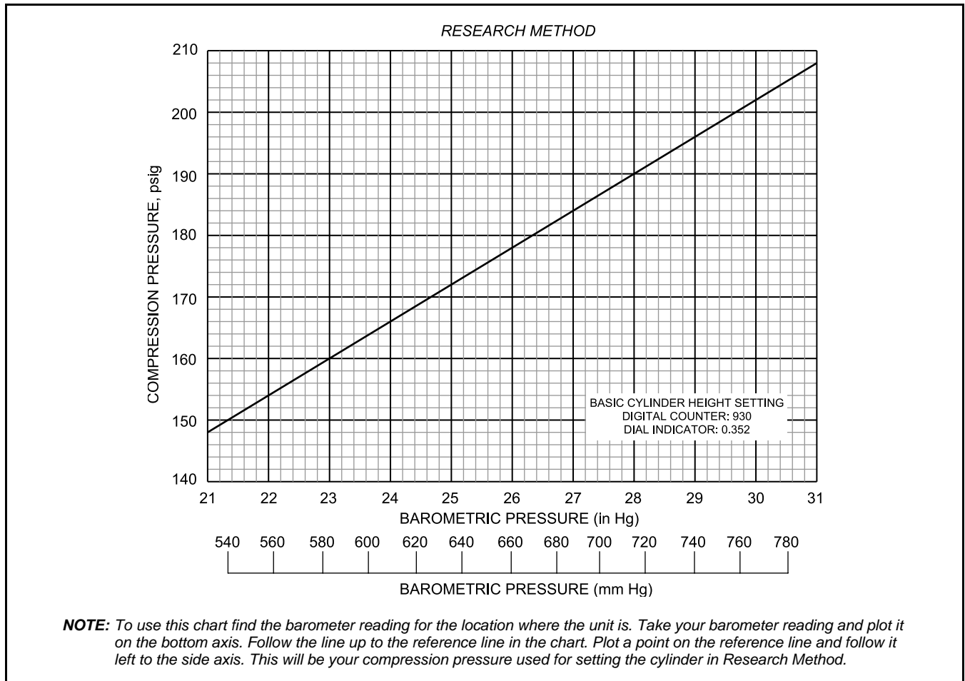
Figure 1. Actual Compression Pressure For Setting Basic Cylinder Height Micrometer Or Digital Counter Assembly For Local Observed Barometric Pressure – Research Method
