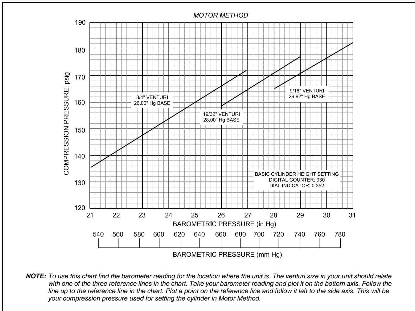
Figure 2. Actual Compression Pressure For Setting Basic Cylinder Height Micrometer Or Digital Counter Assembly For Local Observed Barometric Pressure – Motor Method
